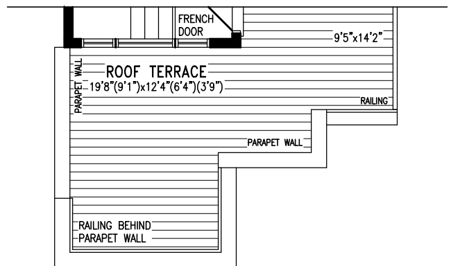
PARTIAL SECOND LEVEL STYLE 'B'
