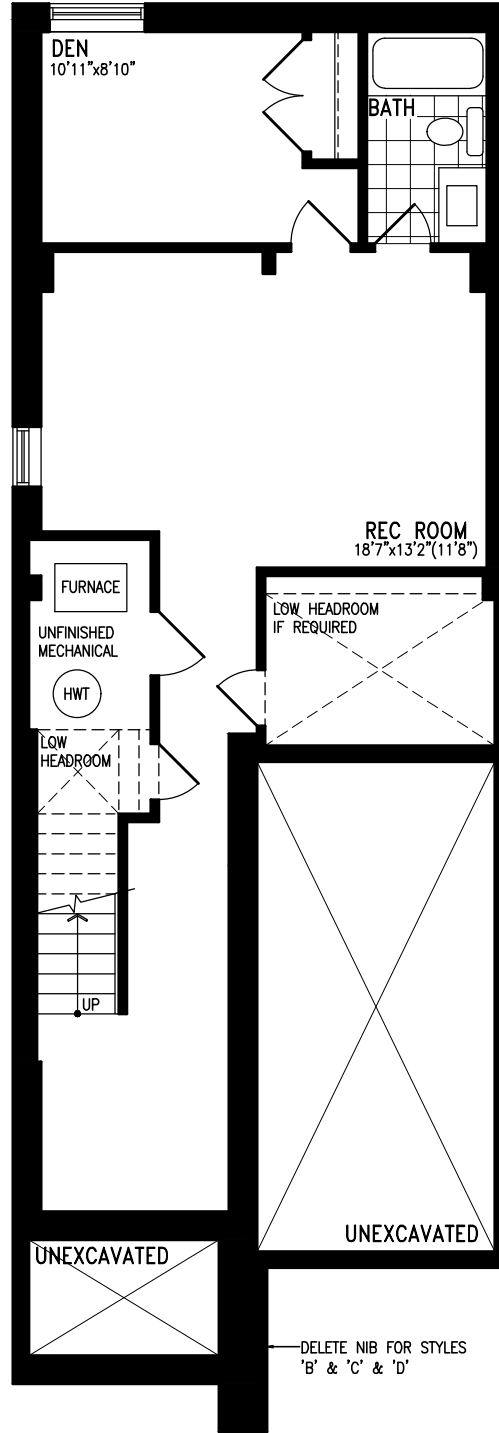
OPT. FINISHED LOWER LEVEL STYLE 'A' & 'B' & 'C' & 'D'
