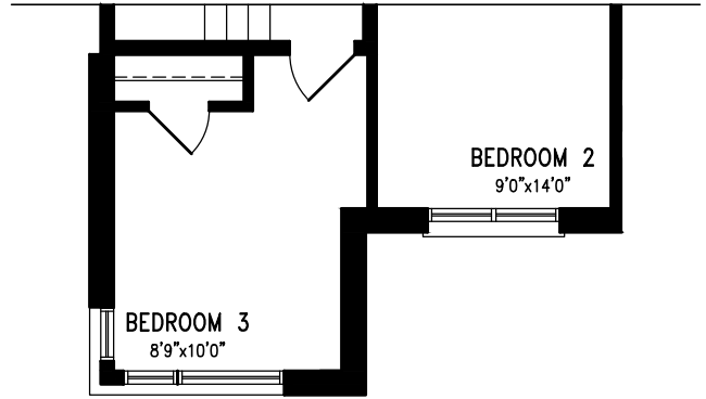
PARTIAL SECOND LEVEL STYLE 'D'
