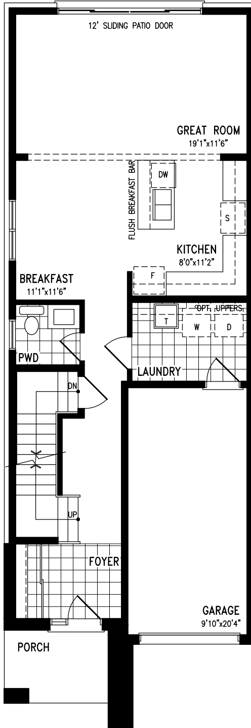
MAIN LEVEL STYLE 'A'
