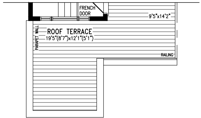
PARTIAL SECOND LEVEL STYLE 'C'
