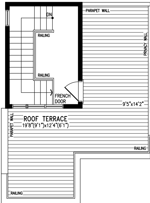
ROOF TERRACE STYLE 'A'
